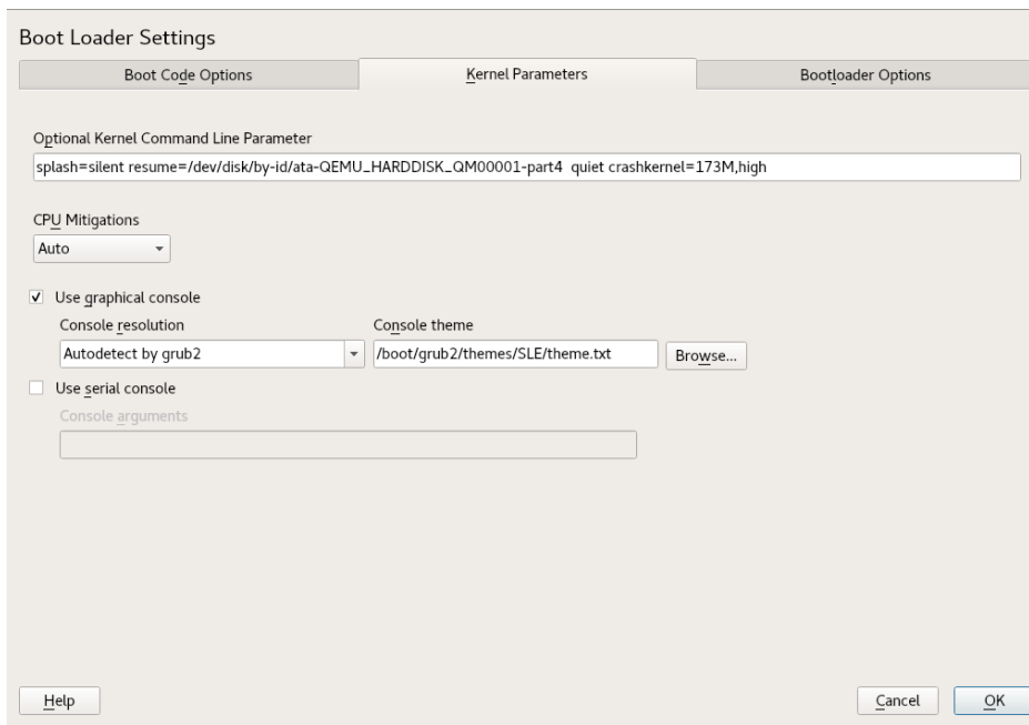
FIGURE 12.5: KERNEL PARAMETERS
