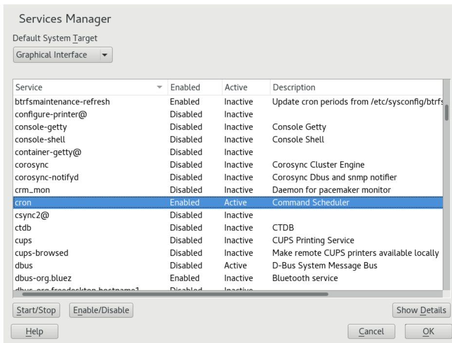
FIGURE 13.1: SERVICES MANAGER
